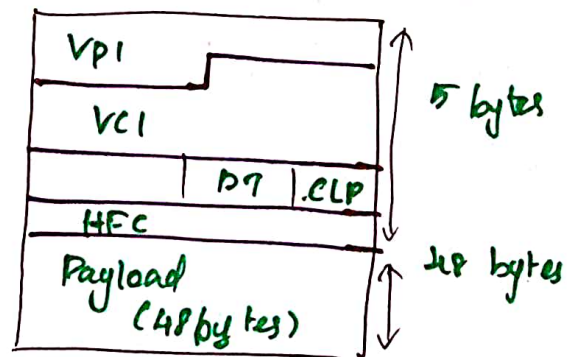
fig NNI cell format
